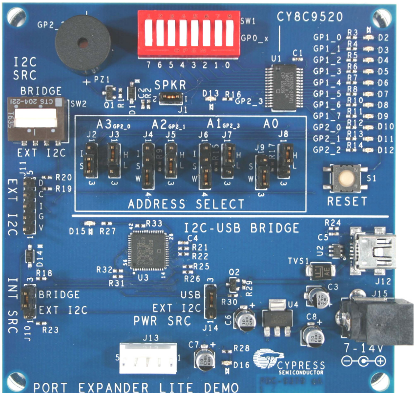
I2C Port Expander Demonstration Board
